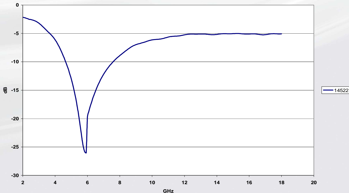
Reflection Loss 14522
