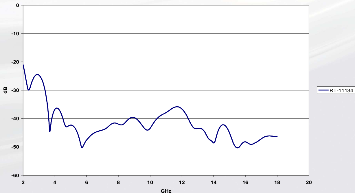
Reflection Loss of RT-11134
