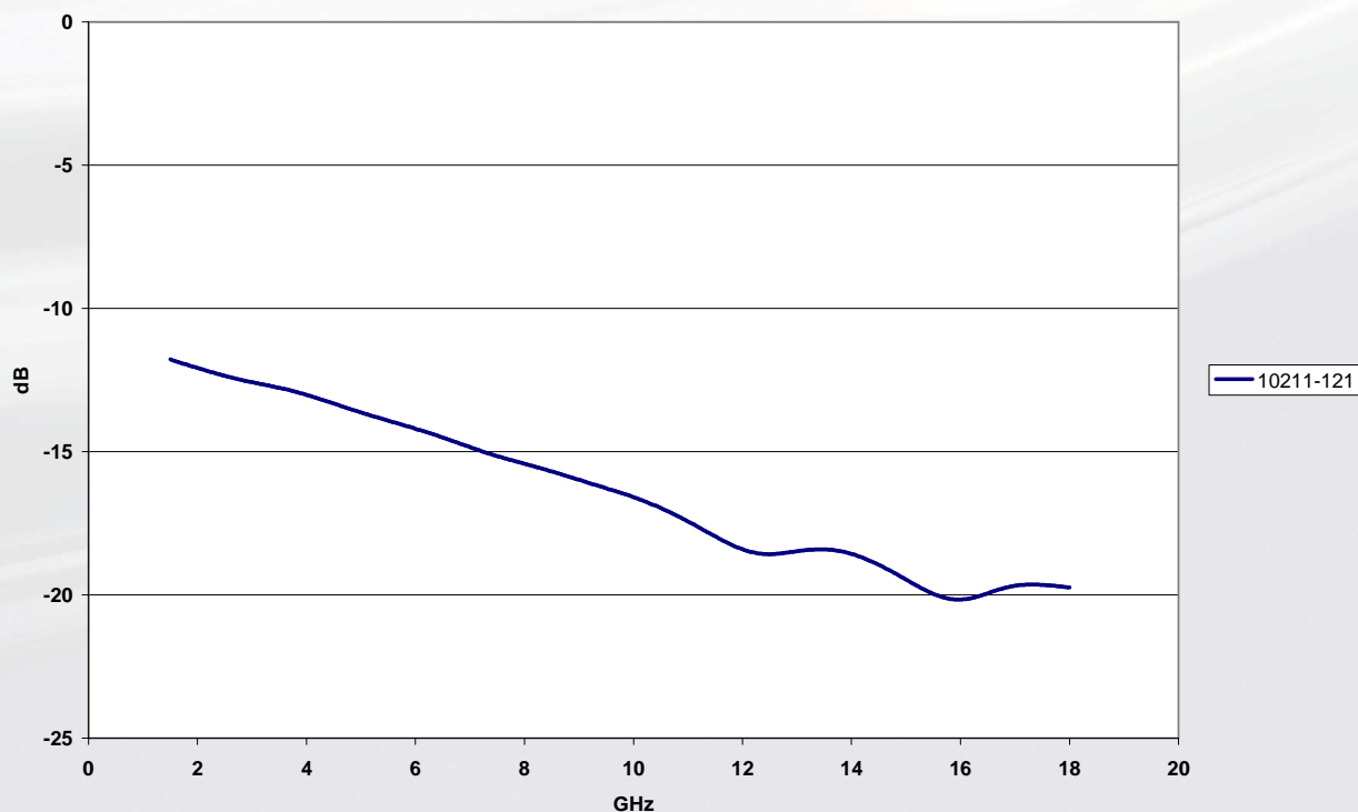
Insertion Loss 10211-121
