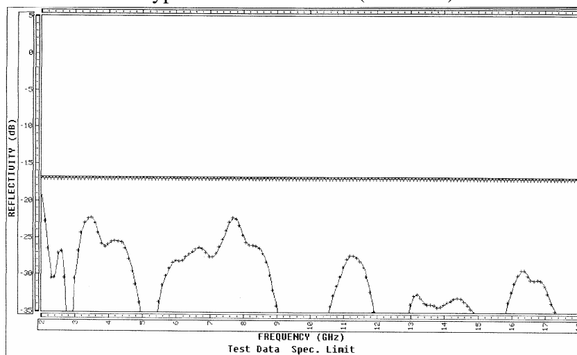
Typical Reflection Loss (2-18GHz):
