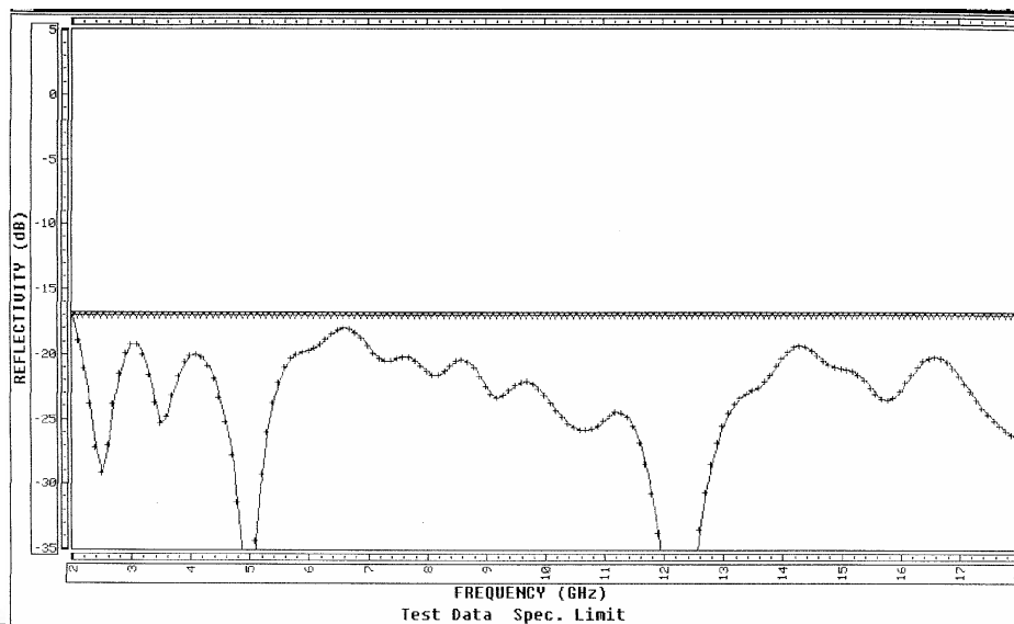
Typical Reflection Loss (2-18GHz):
